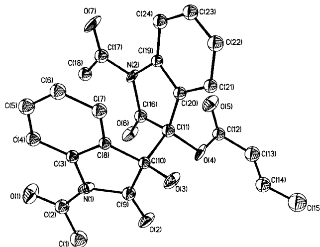
Figure 1. X-ray structure of 6a
