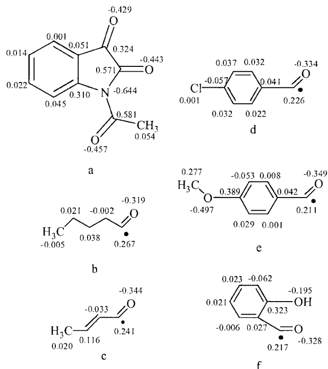
Figure 2. Atomic charges in: (a) ground state 1 , (b) valeroyl radical, (c) crotonyl radical, (d) p -chlorobenzoyl radical, (e) p -methoxybenzoyl radical, and (f) o -hydroxybenzoyl radical (charge density at the hydrogen atom has been summed up to their attached carbon atom)
